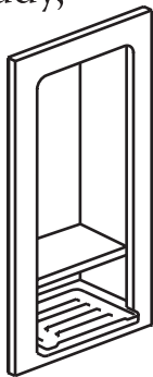
Cut-out 6 3/4" w 13 3/4" h
