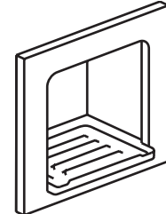
Cut-out 6 3/4" w 5 7/8" h 3 1/2" d
